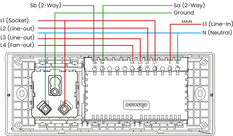
Figure 1: Wiring Diagram - 1-Way Installation
